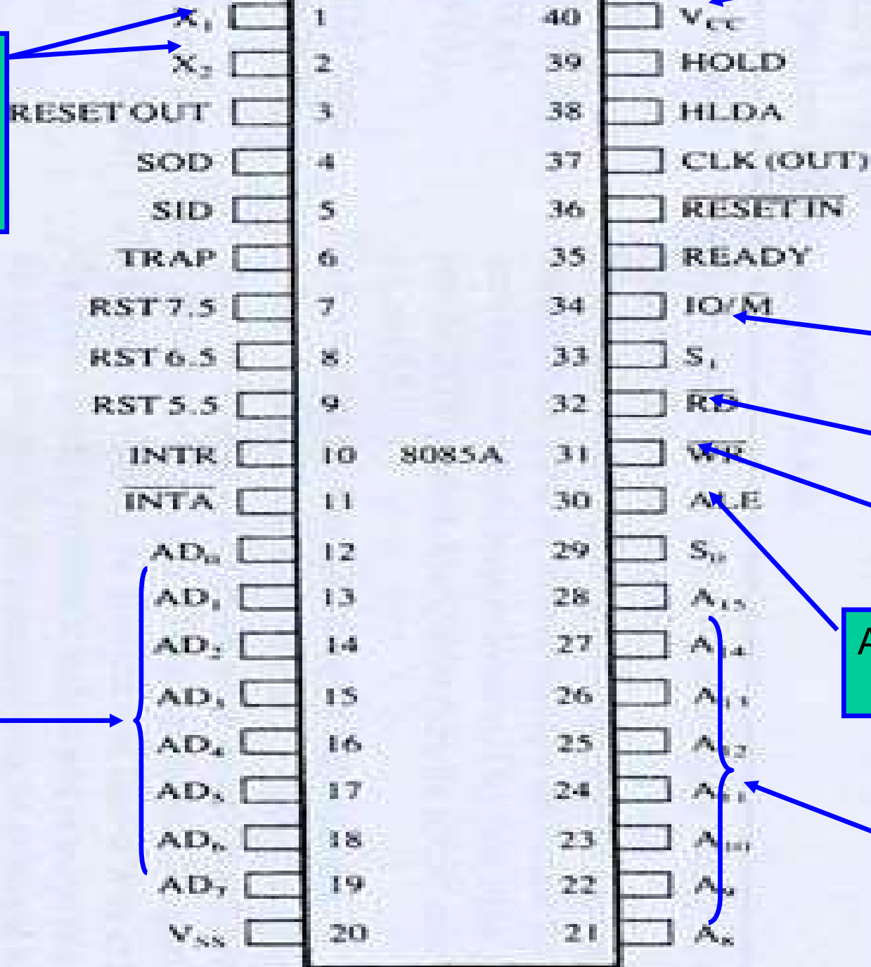
8085 Pinout
